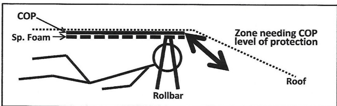
Figure 5, Zone of vehicle needing COP level of protection as per 4.10.2
